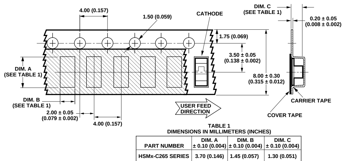
Figure 16. Tape dimensions.
