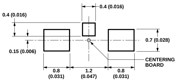
Figure 9. Recommended soldering pattern for HSMx-C120.
