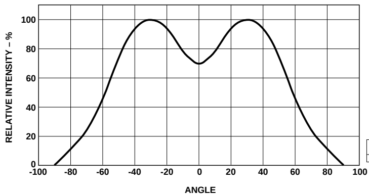
Figure 5c. Relative intensity vs. angle for HSMx-C110.
