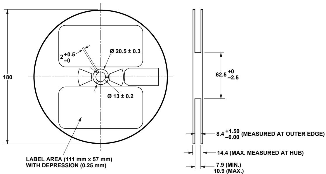
Figure 12. Reel dimension.
