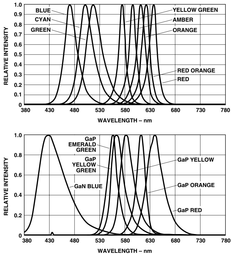
Figure 1. Relative intensity vs. wavelength.
