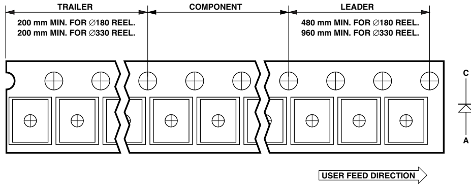
Figure 10. Tape leader and trailer dimension.
