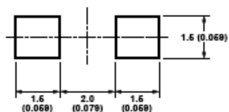
Figure 11. Recommended soldering pattern for HSMx-C150.
