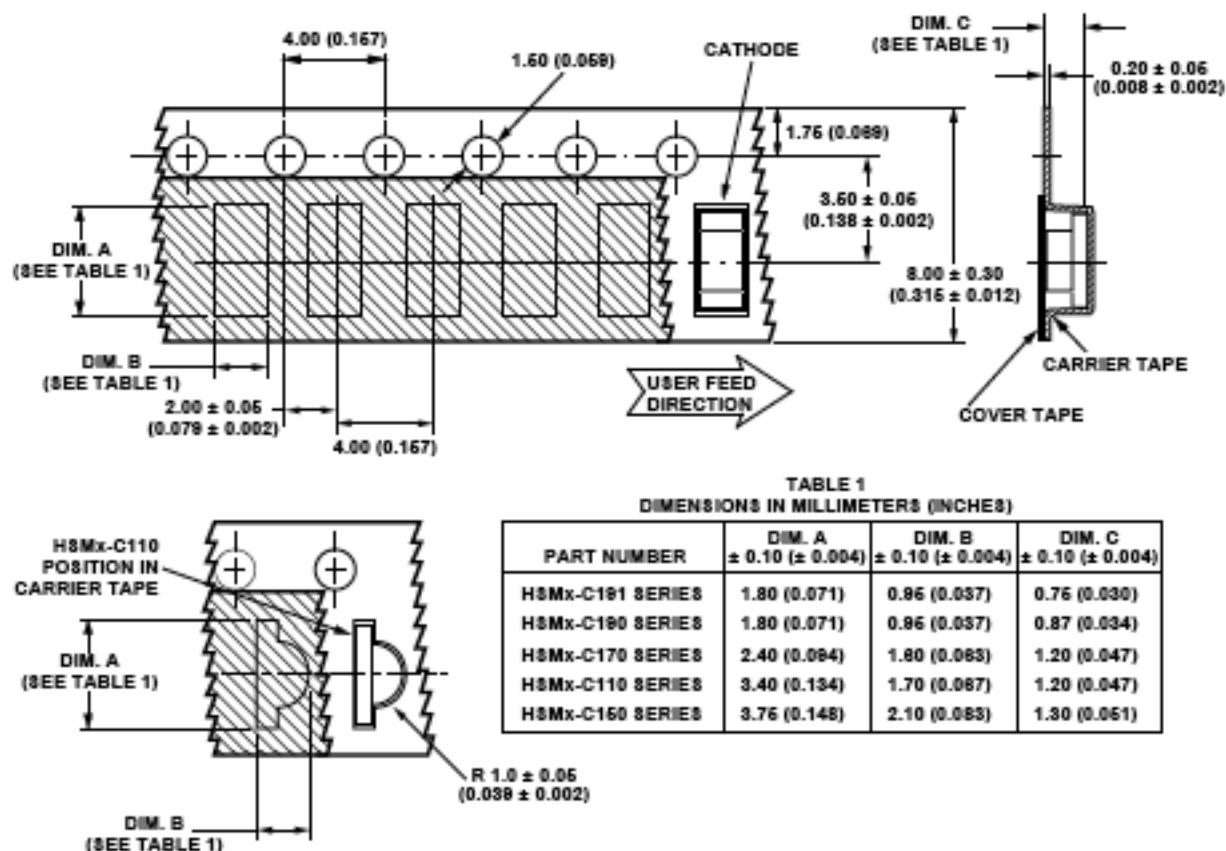
Figure 14. Tape dimensions.
