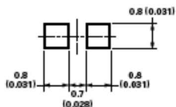
Figure 10. Recommended soldering pattern for HSMx-C190 and HSMx-C191.
