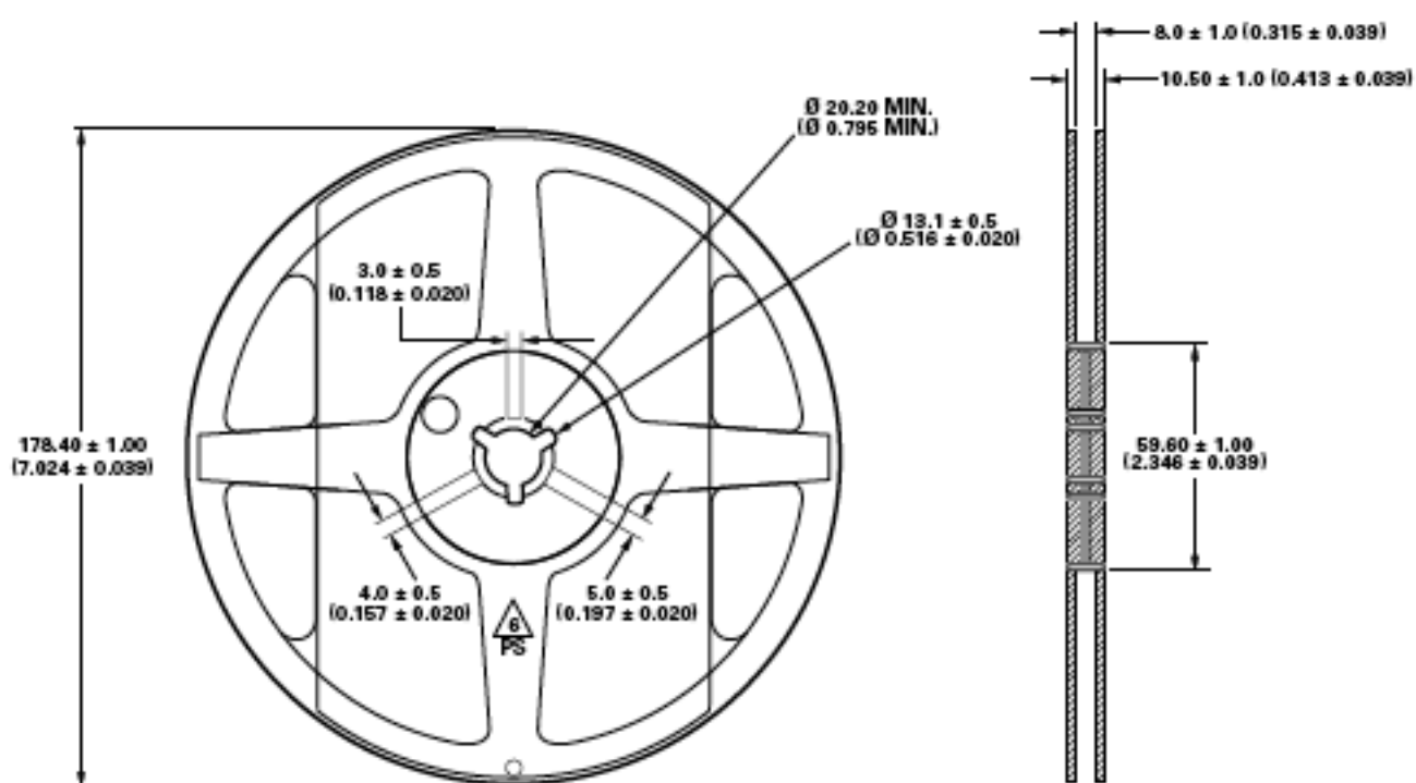
Figure 13. Reel dimensions.
