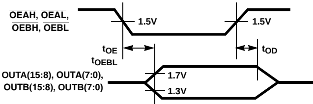
FIGURE 53. OUTPUT ENABLE/DISABLE
