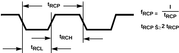
FIGURE 55. REFCLK
