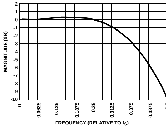
FIGURE 15. POLYPHASE RESAMPLER FILTER EXPANDED RESOLUTION PASSBAND FREQUENCY RESPONSE
