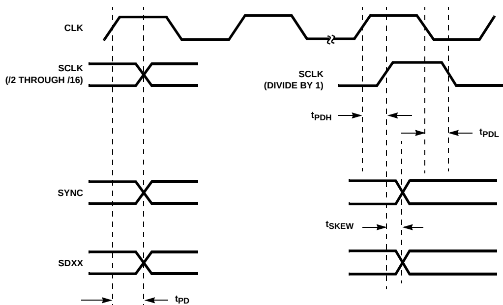
FIGURE 6. SERIAL OUTPUT TIMING
