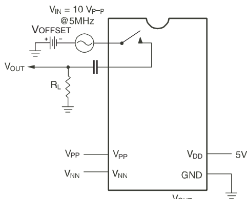
OFF Isolation
