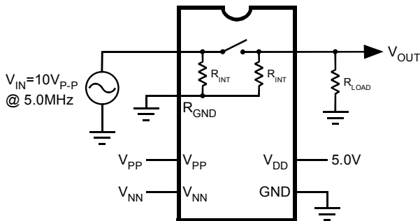
Off Isolation
