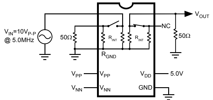
Crosstalk
