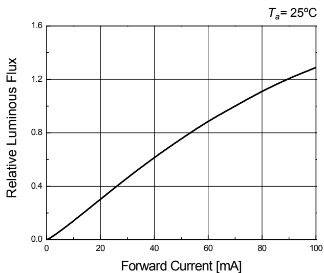
Forward Current vs. Relative Flux
