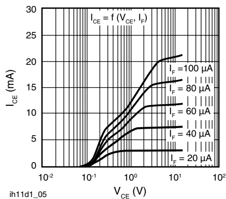
Fig. 4 - Output Characteristics
