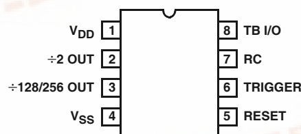
ICM7242 (8 LD PDIP, SOIC) TOP VIEW
