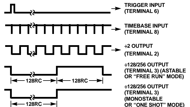
FIGURE 1. TIMING DIAGRAMS OF OUTPUT WAVEFORMS FOR THE ICM7242 (COMPARE WITH FIGURE 5)
