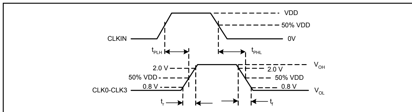
Figure 2. Voltage Thresholds for Propagation Delay ( t_{pd} ) Measurements
