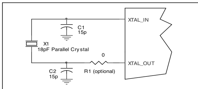
FIGURE 2. CRYSTAL OSCILLATOR INTERFACE
