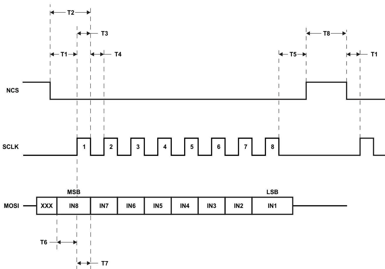
Figure 1. Serial Communications
