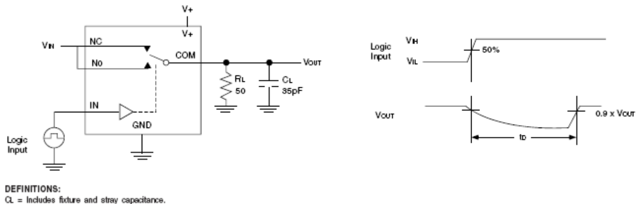
Break-Before-Make Interval
