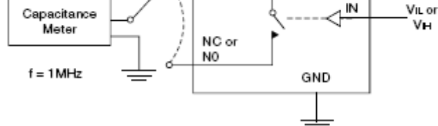
Channel Off/On Capacitance
