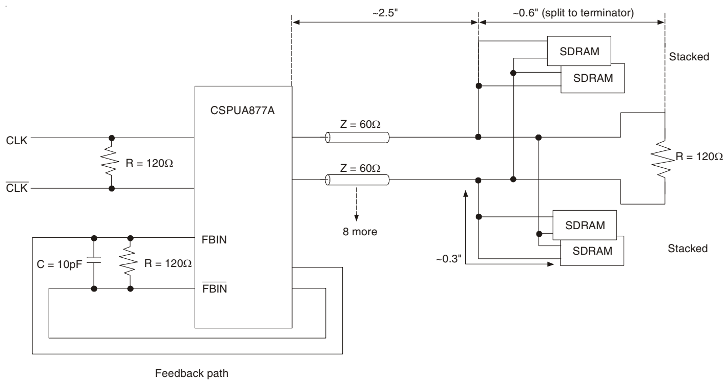
Clock Structure 2
