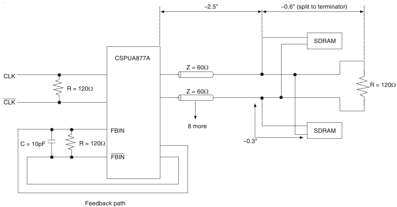
Clock Structure 1
