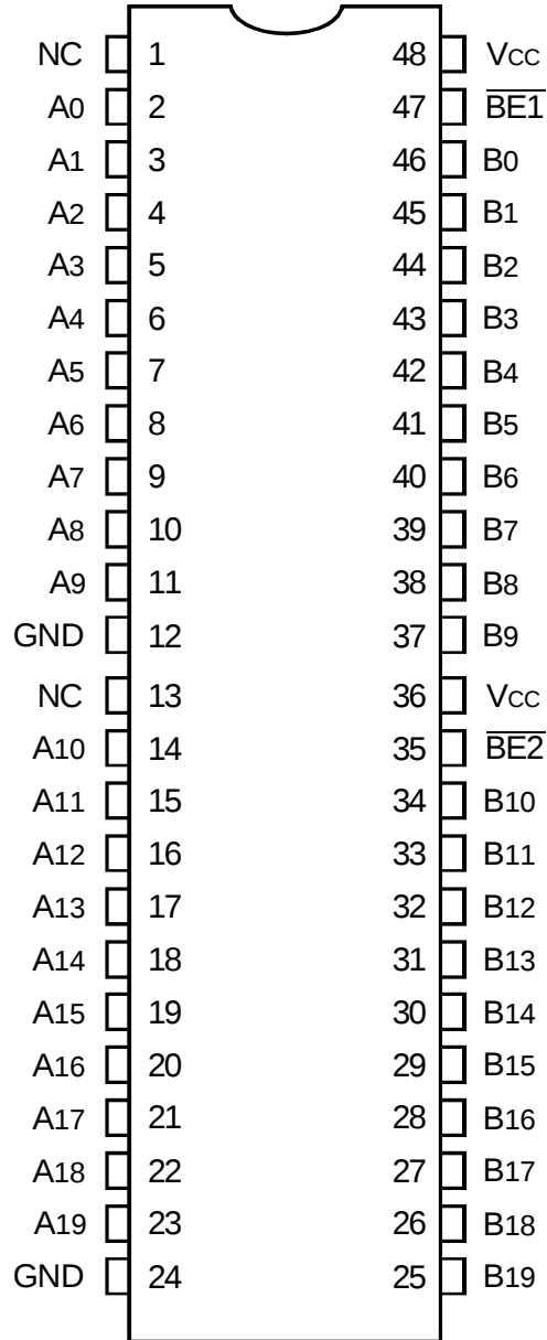
SSOP/ TSSOP TOP VIEW
