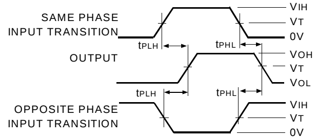
Propagation Delay
