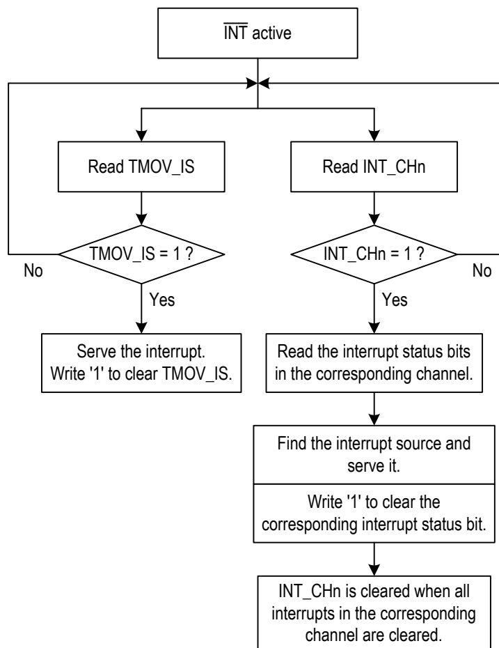
Figure-44 Interrupt Service Process
