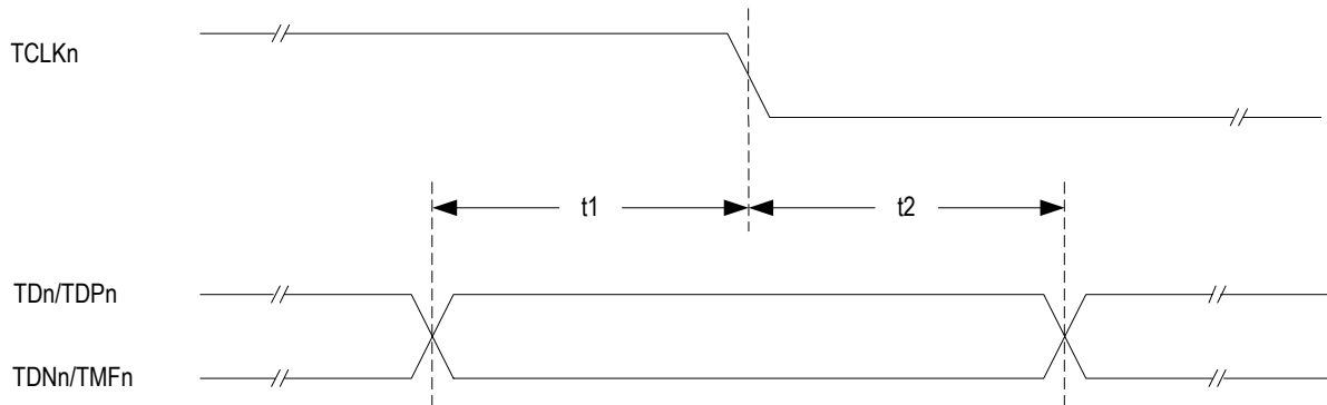
Figure-51 Transmit Clock Timing Diagram
