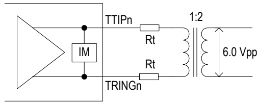
Figure-19 Transmit Differential Line Interface with Twisted Pair Cable (with Transformer)
