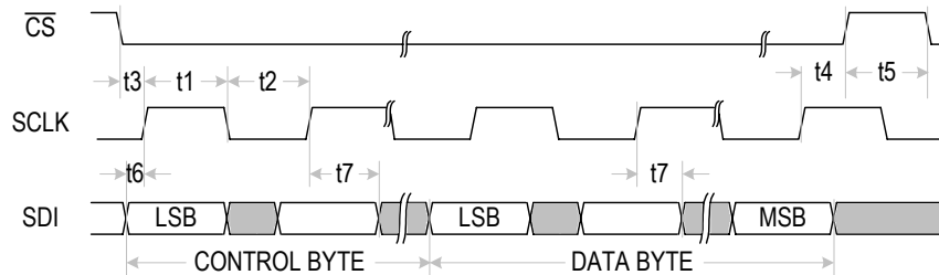
Figure-36 Serial Interface Write Timing
