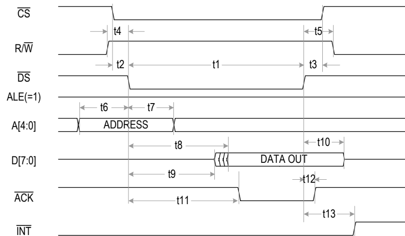
Figure-32 Non-Multiplexed Motorola Mode Read Timing
