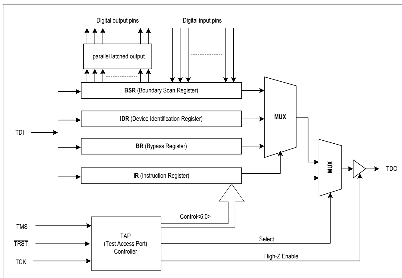
Figure-12 JTAG Architecture
