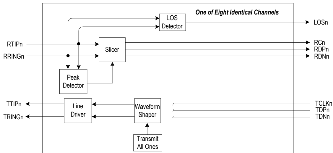
Figure-8 TAOS Data Path
