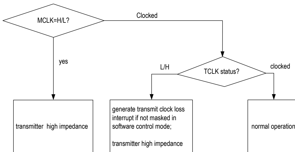
Figure-16 TCLK Operation Flowchart
