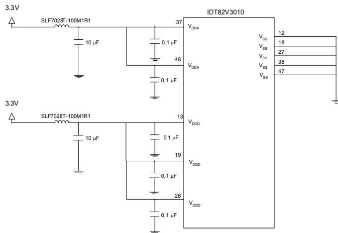
Figure - 10 IDT82V3010 Power Decoupling Scheme
