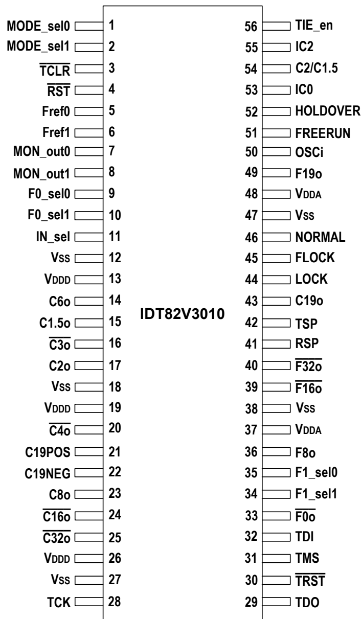
Figure - 1 IDT82V3010 SSOP56 Package Pin Assignment
