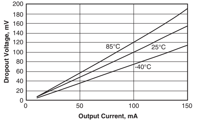
Dropout Voltage vs. I OUT
