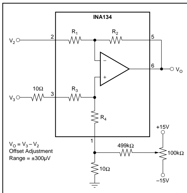
FIGURE 2. Offset Adjustment.
