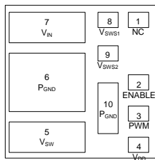
BOTTOM VIEW ELECTRICAL I/O
