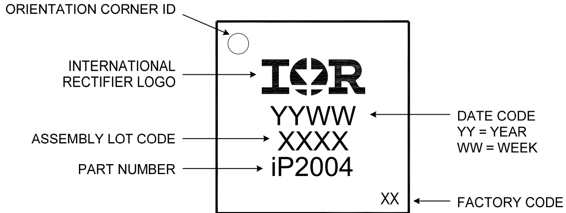
Figure 19 Part Marking
