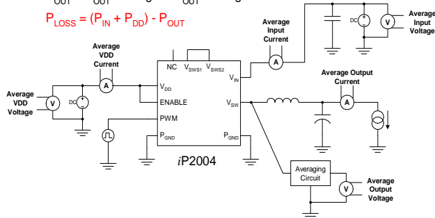
Figure 9 Power Loss Test Circuit
