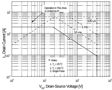
Figure 9-1. Maximum Safe Operating Area for IRF710B
