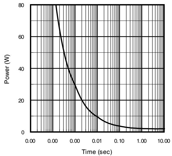
Fig 8. Typical Power Vs. Time
