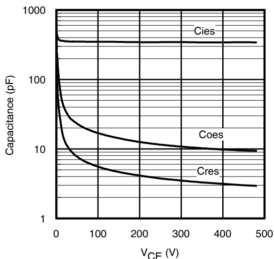
Fig. 23- Typ. Capacitance vs. V_{CE}
