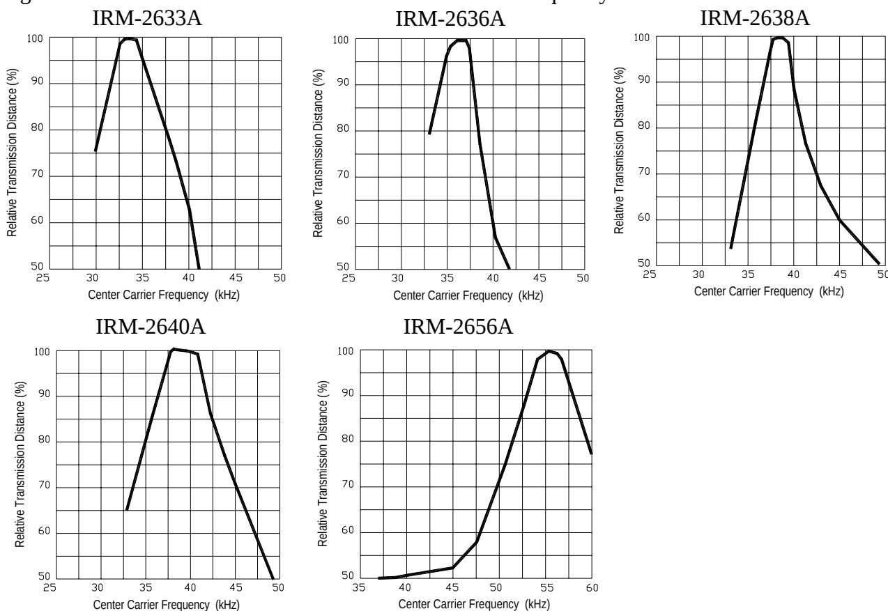
Fig.-9 Relative Transmission Distance vs. Center Carrier Frequency
