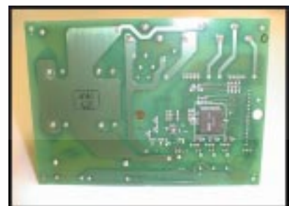
IRMDAC3 Host PCB Bottom Layer
