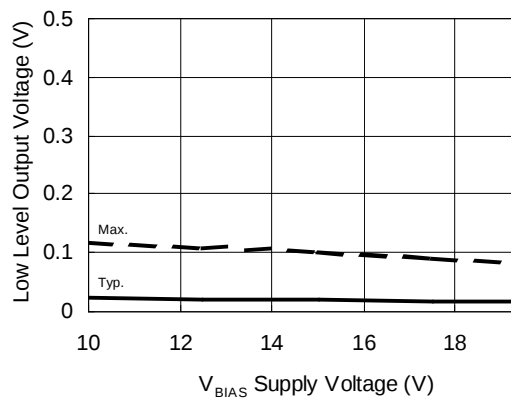
Figure 15B. Low level Output vs. Supply Voltage
