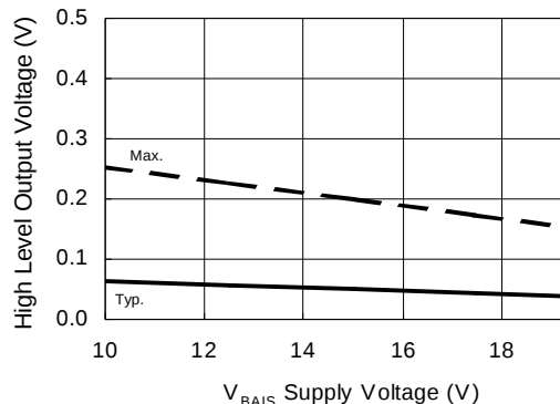
Figure 14B. High Level Output vs. Supply Voltage
