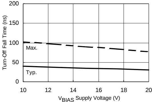
Figure 10B. Turn-Off Fall Time vs. Voltage
