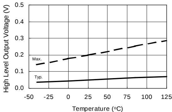
Figure 14A. High Level Output Voltage vs. Temperature
