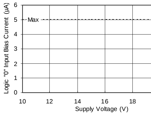
Figure 13B. Logic "0" Input Bias Current vs. Voltage
