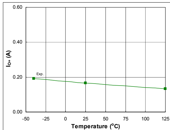
Figure 08: I_{O+} vs. temperature
