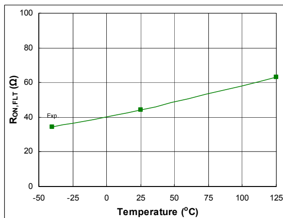
Figure 59: R_{ON,FLT} vs. temperature
