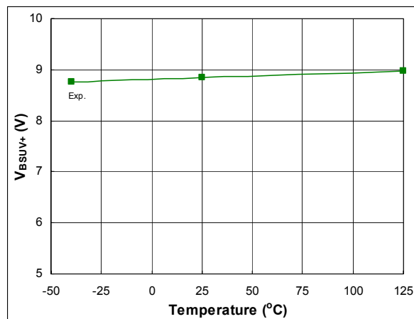
Figure 54: V_{BSUV+} vs. temperature
