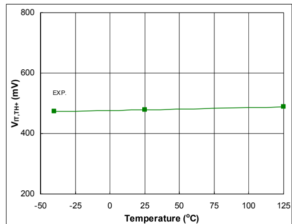
Figure 56: V_{IT,TH+} vs. temperature
