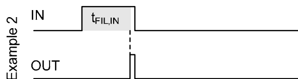
Figure 17: Typical input filter
