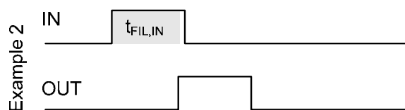
Figure 18: Advanced input filter
