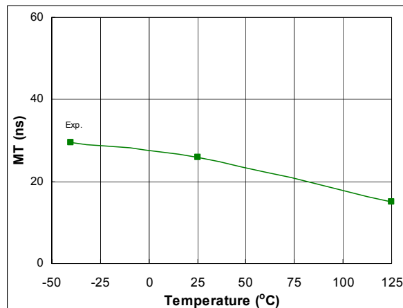
Figure 44: MT vs. temperature
