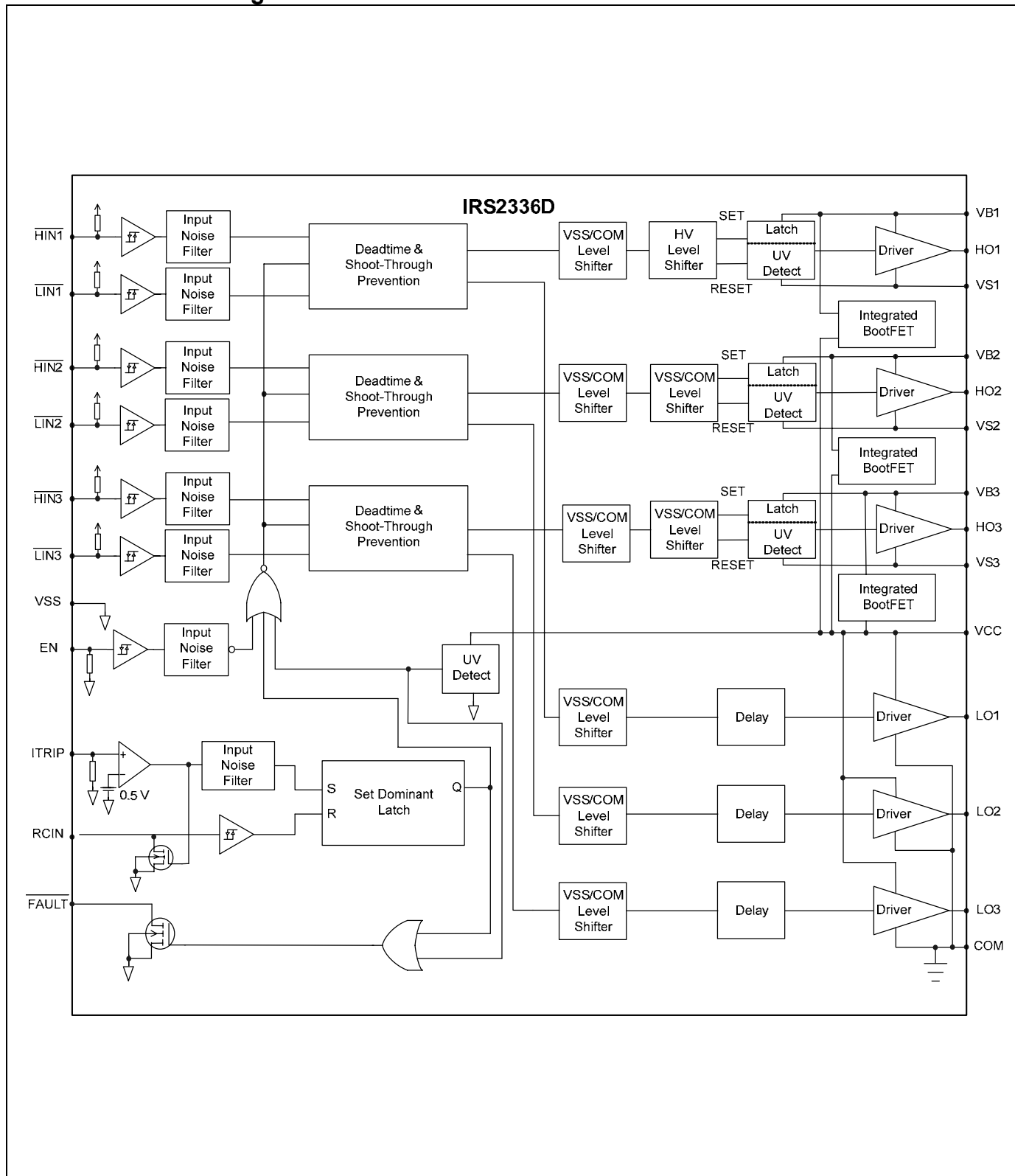
Functional Block Diagram: IRS2336D
