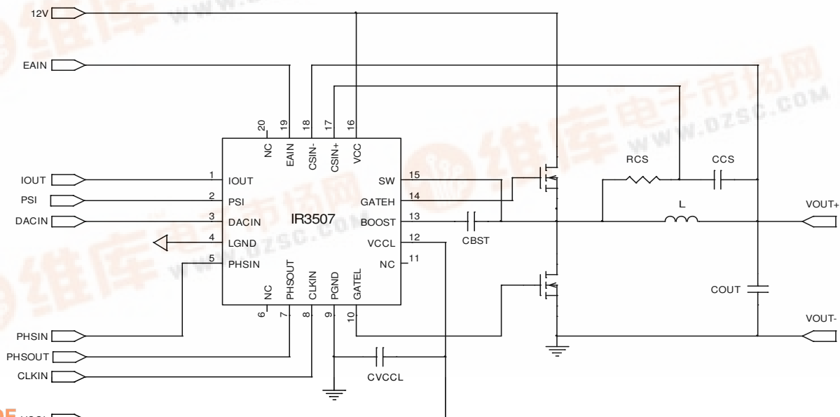
Figure 1 Application Circuit
