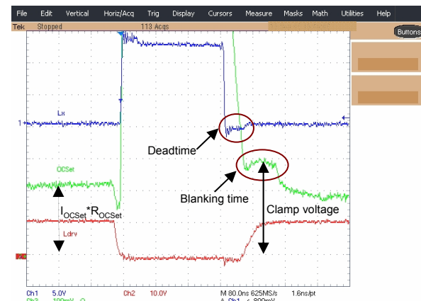
Fig. 9: OCSet pin during normal condition Ch1: Inductor point, Ch2:Ldrv, Ch3:OCSet
