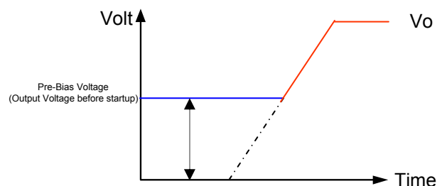
Fig. 4: Pre-Bias startup
