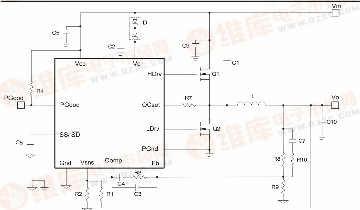
Fig. 1: Typical application Circuit
