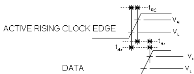
Timing For I 2 S Receiver
