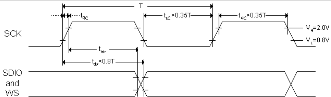
Timing For I 2 S Transmitter
