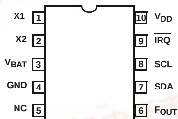
ISL1220 (10 LD MSOP) TOP VIEW
