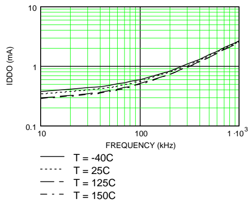
FIGURE 6. ISL2101A IDD OPERATING CURRENT vs FREQUENCY
