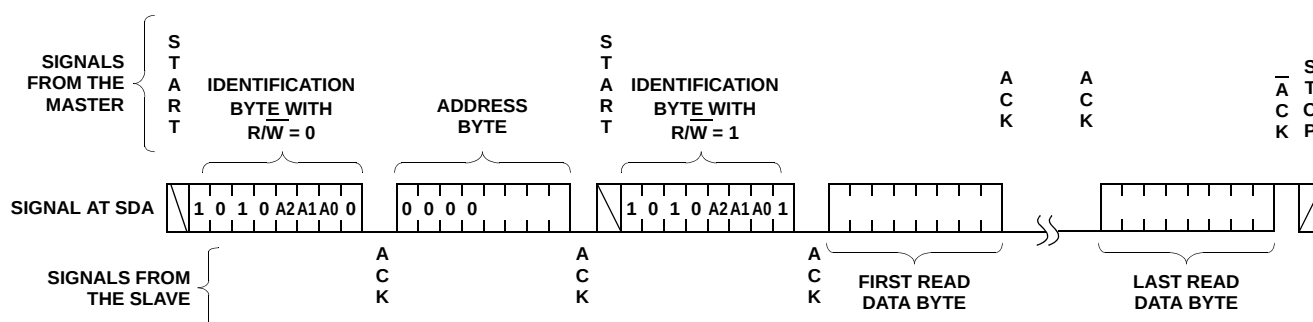
FIGURE 15. READ SEQUENCE
