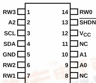
ISL22349 (14 LD TSSOP) TOP VIEW
