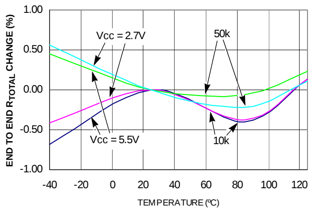
FIGURE 9. END TO END R_{\text{TOTAL}} % CHANGE vs TEMPERATURE
