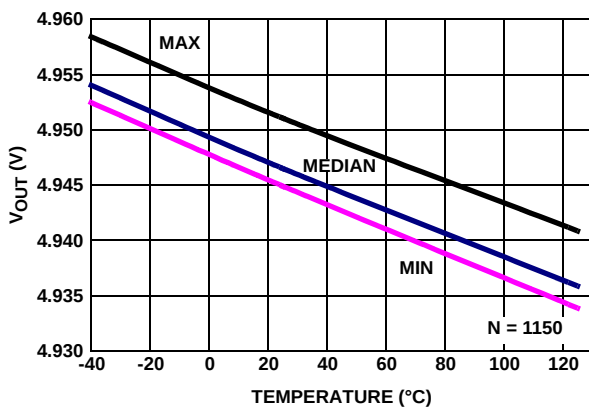
FIGURE 34. V_{OUT} HIGH vs TEMPERATURE V_+ , V_- = \pm 2.5V , R_L = 1k
