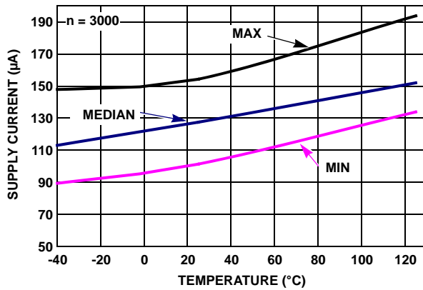
FIGURE 21. ISL28271 SUPPLY CURRENT ENABLED vs TEMPERATURE, V_+ = \pm 2.5V , V_{IN} = 0V
