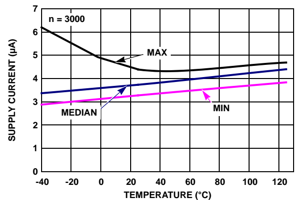
FIGURE 24. ISL28272 SUPPLY CURRENT DISABLED vs TEMPERATURE, V_+ = \pm 2.5V , V_{IN} = 0V
