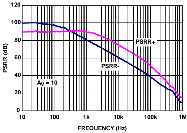
FIGURE 13. ISL28271 PSRR vs FREQUENCY
