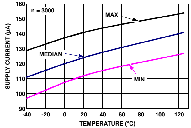
FIGURE 22. ISL28272 SUPPLY CURRENT ENABLED vs TEMPERATURE, V_+ = \pm 2.5V , V_{IN} = 0V
