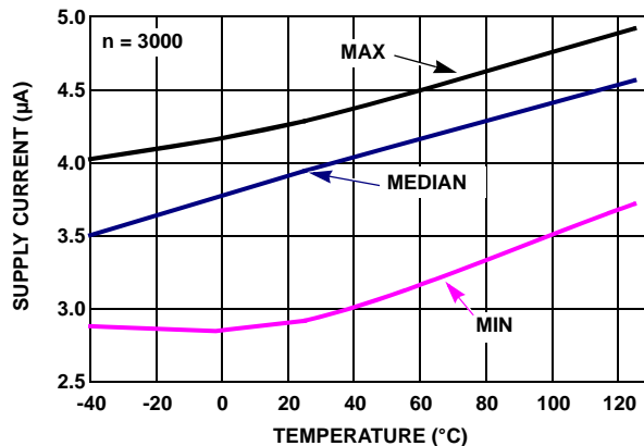
FIGURE 23. ISL28271 SUPPLY CURRENT DISABLED vs TEMPERATURE, V_+ = \pm 2.5V , V_{IN} = 0V
