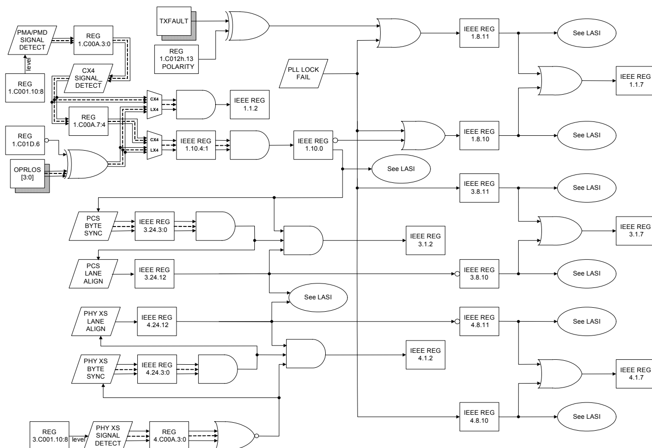
FIGURE 4. IEEE AND VENDOR SPECIFIC FAULT AND STATUS REGISTERS (EQUIVALENT SCHEMATIC)
