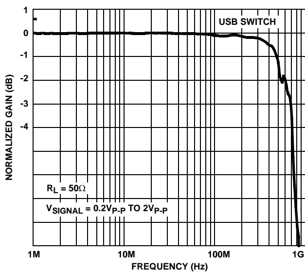
FIGURE 14. FREQUENCY RESPONSE
