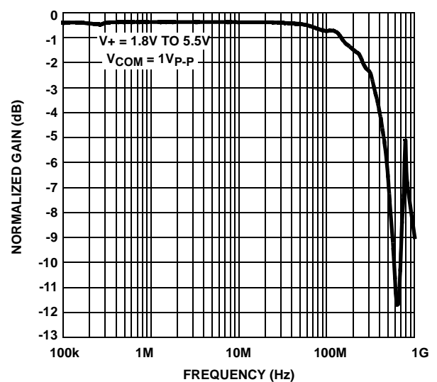
FIGURE 15. FREQUENCY RESPONSE
