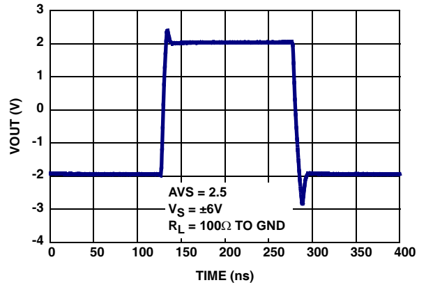
FIGURE 16. LARGE SIGNAL STEP RESPONSE - VCM TO V OUT
