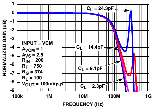
FIGURE 7. VCM GAIN vs FREQUENCY vs CL
