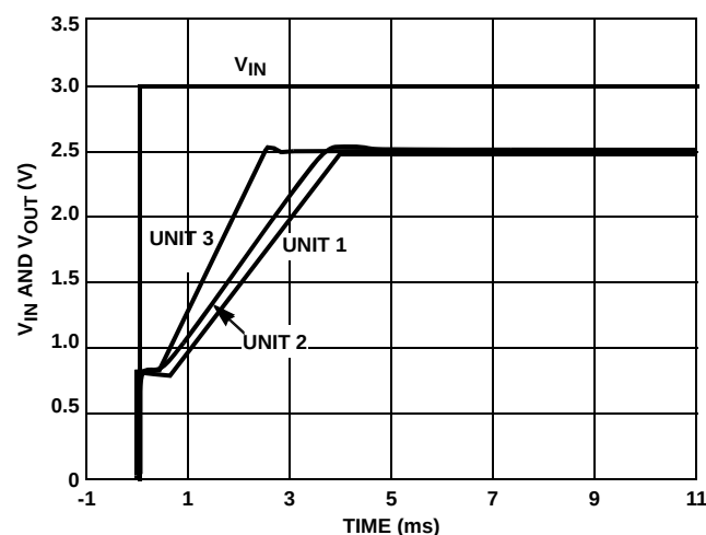
FIGURE 119. TURN-ON TIME
