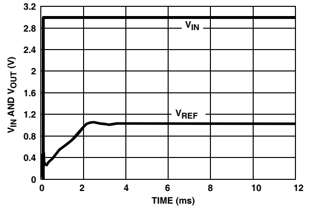
FIGURE 12. TURN-ON TIME ( +25^{\circ}C )
