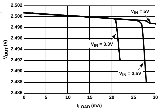
FIGURE 114. DIFFERENT V_{IN} AT ROOM TEMPERATURE
