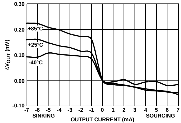
FIGURE 36. LOAD REGULATION
