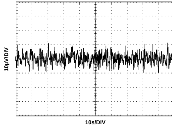
FIGURE 82. V_{OUT} NOISE
