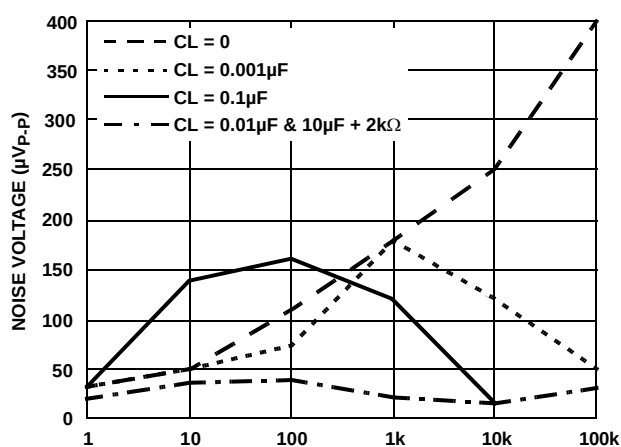
FIGURE 117. NOISE REDUCTION
