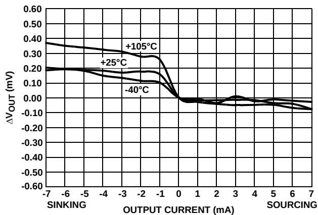
FIGURE 106. LOAD REGULATION
