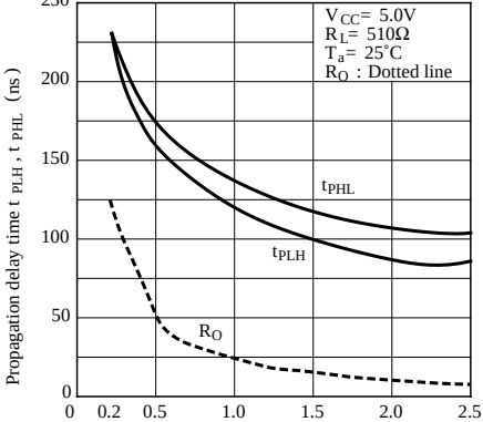
Fig. 9 Propagation Delay Time vs. Incident Light Intensity
