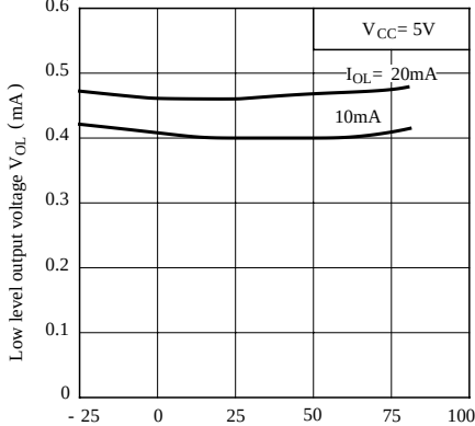
Fig. 3 Low Level Output Voltage vs. Ambient Temperature
