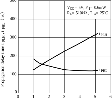
Fig.10 Propagation Delay Time vs. Gain Resistance
