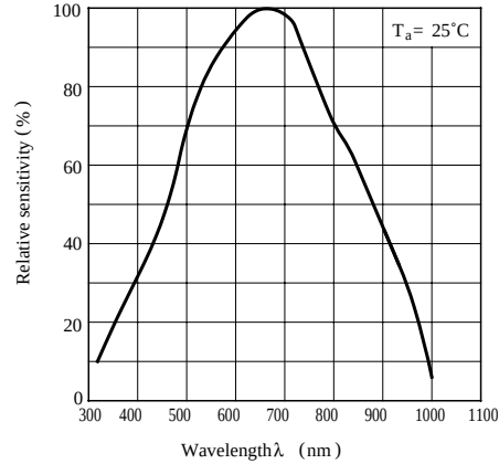
Fig.14 Spectral Sensitivity
