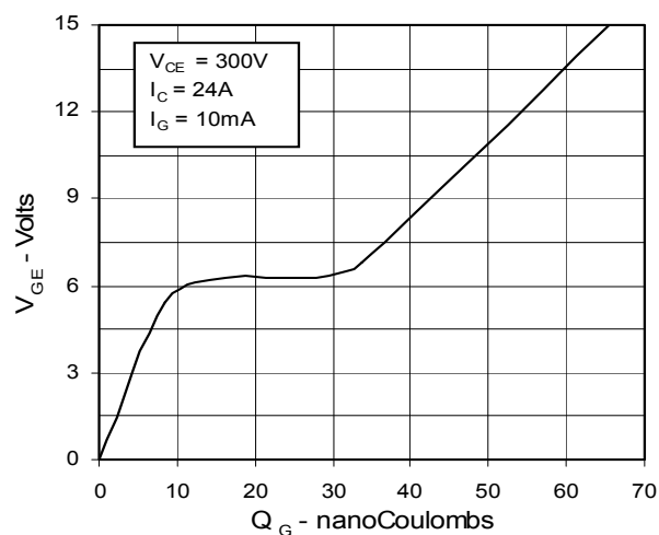
Fig. 14. Gate Charge
