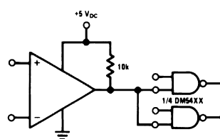
Driving TTL
