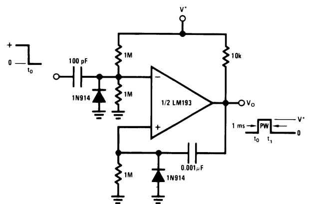
One-Shot Multivibrator
