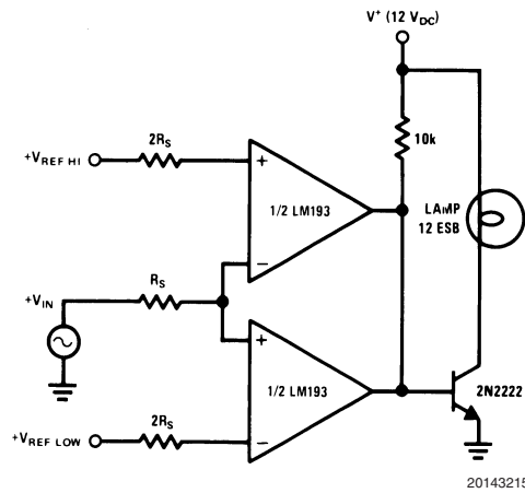
Limit Comparator
