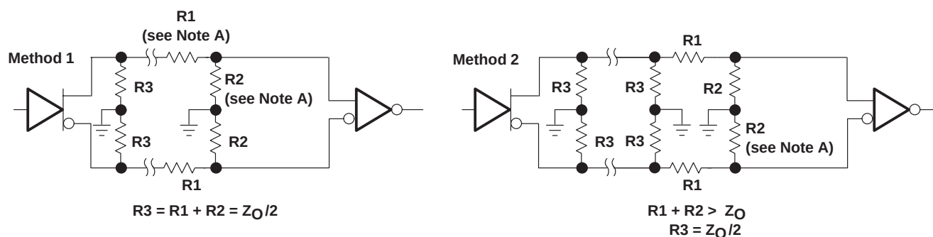
Figure 16. Termination Techniques
