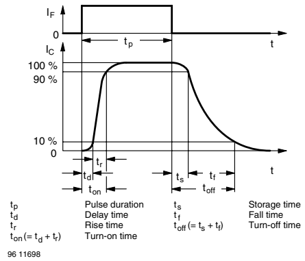
Fig. 3 - Switching Times
